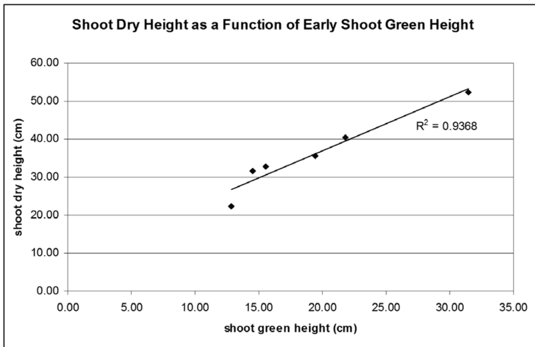
Figure 4. Shoot dry height (SDH) as a function of early shoot green height. The two markers are highly correlated ( r^2 = 0.9368 ). Early shoot green height predicts SDH, so serves as an indicator of vigor with respect to water stress.
